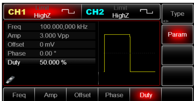
Square wave with 50% duty cycle
