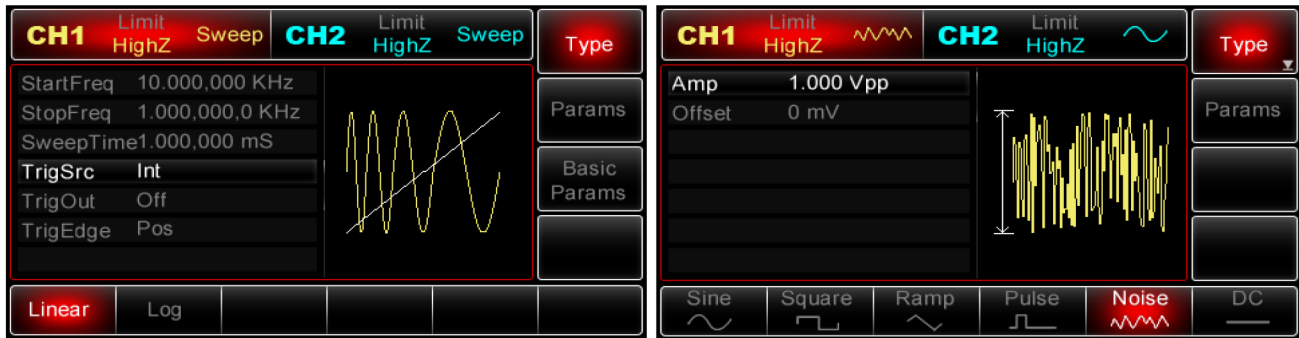
Sweep function and burst mode
